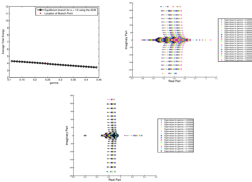
FIGURE 3. Plot of the lowest equilibrium branch constructed using the adjoint continuation method (top left) of [1] with \eta = 1 , \alpha_1 = 0.5 , \alpha_2 = 1.0 along with two plots of the spectrum of the linearized forward problem, for \gamma > .25 (top right) and \gamma < .25 (bottom). The fact that the spectrum moves to the positive real part is evidence of a branch bifurcation happening near \gamma = .25 in the numerical continuation.
