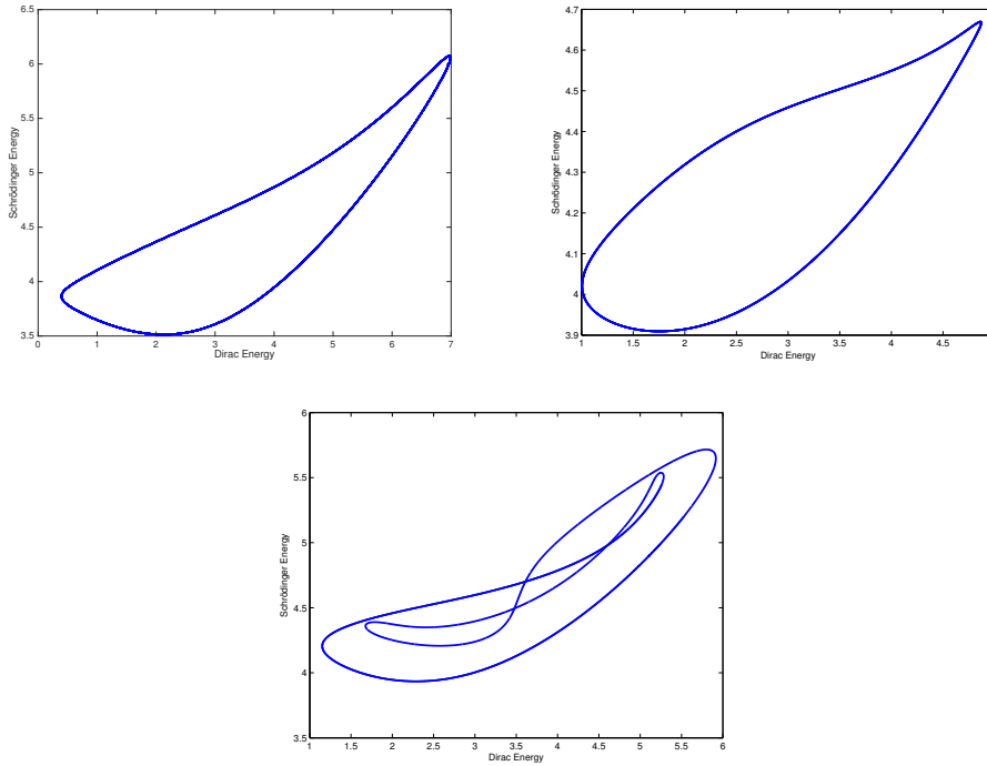
FIGURE 4. Top Left: Plot of the Dirac Final Energy versus Schrödinger Final Energy in the case of a periodic solution from the branch of periodic solutions in Figure 2 with \gamma = .4 . Top Right: Plot of the Dirac Final Energy versus Schrödinger Final Energy in the case of a solution from the period doubling branch in Figure 2 with \gamma = .4 . Bottom: Plot of the Dirac Final Energy versus Schrödinger Final Energy in the case of a solution from the period doubling branch in Figure 1 with \gamma = .373 .
